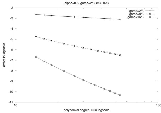
Figure 6: B^{0.25} -errors versus N with M = 15 for varying \gamma .
