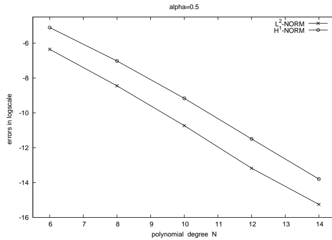
Figure 3: H^1 - and L^2 -errors versus N with M = 15 , \alpha = 0.5 .
