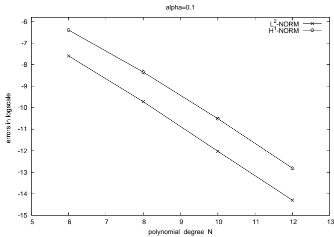
Figure 2: H^1 - and L^2 -errors versus N with M = 15 , \alpha = 0.1 .
