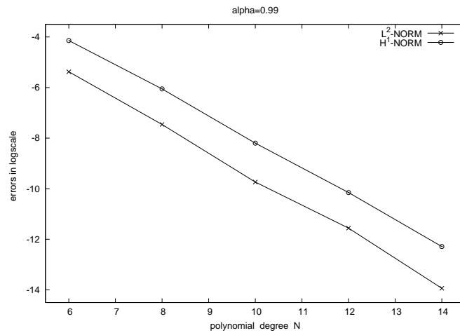
Figure 4: H^1 - and L^2 -errors versus N with M = 15 , \alpha = 0.99 .
