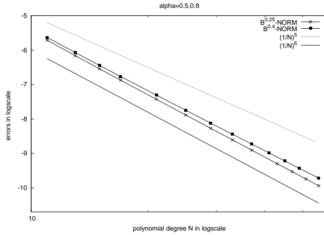
Figure 5: B^{\alpha/2} -errors versus N with M = 15 , \alpha = 0.5, 0.8 for the solution of limited regularity.
