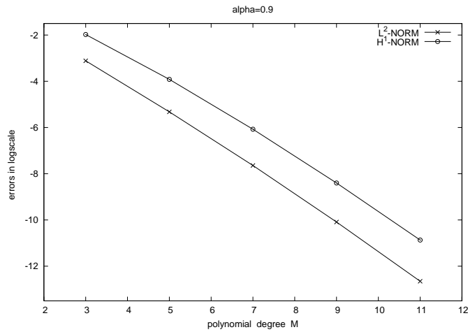
Figure 1: H^1 - and L^2 -errors versus M with N = 16 , \alpha = 0.9 .
